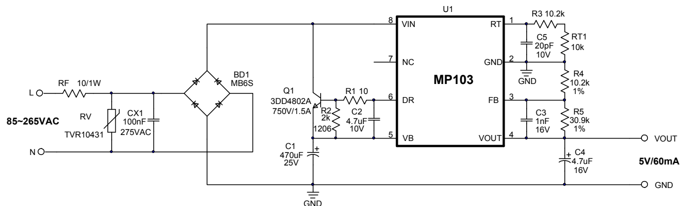
Figure 7: Typical Application
