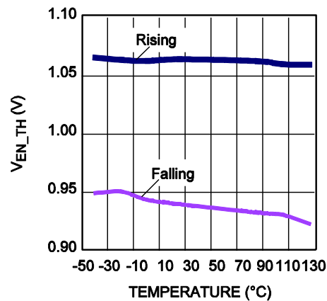
EN Threshold vs. Temperature
