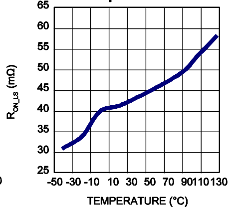
LS-FET On Resistance vs. Temperature
