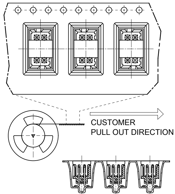
VIEW FOR 1 SIDE PILOT HOLE
