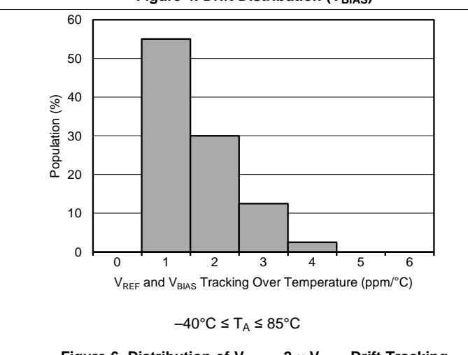
Figure 6. Distribution of V_{REF} - 2 \times V_{BIAS} Drift Tracking Over Temperature
