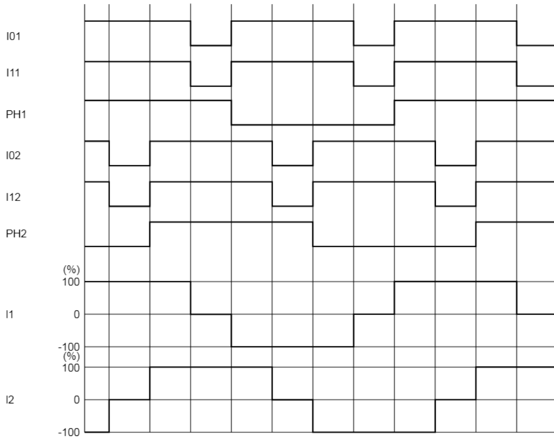
Half step full torque (CW mode)
