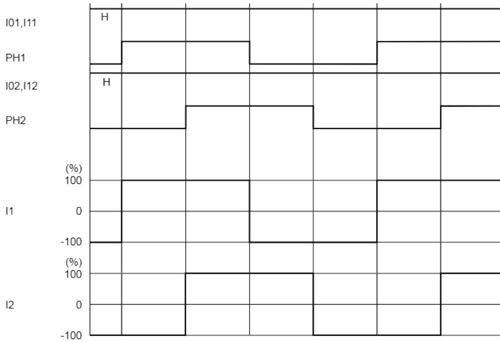
3-4) Typical current waveform in each excitation mode when stepping motor parallel input control Full step (CW mode)
