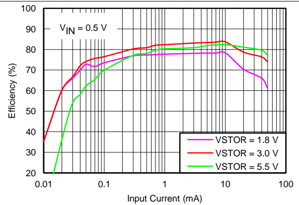
V_{IN} = 0.5 \text{ V} V_{IN\_DC} = sourcemeter configured with voltage source = 0.5 V and I_{COMP} varied from 0.01 mA to 100 mA V_{STOR} = sourcemeter configured to measure current and voltage source set to hold the V_{STOR} voltage = 1.8 V, 3.0 V or 5.5 V
