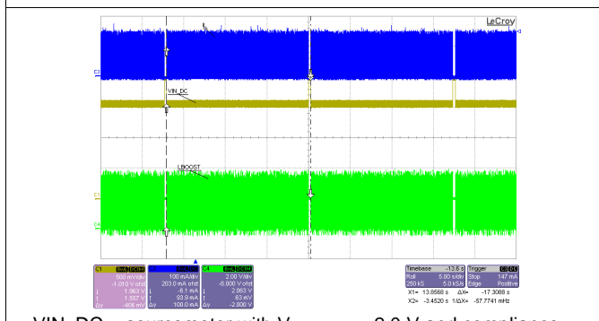
V_{IN\_DC} = sourcemeeter with V_{SOURCE} = 2.0\text{ V} and compliance of 43\text{ mA} V_{BAT} = sourcemeeter with V_{SOURCE} = 3.0\text{ V} and compliance of 1\text{ A}
