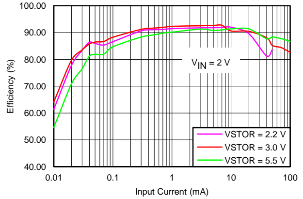
V_{IN} = 2 \text{ V} V_{IN\_DC} = sourcemeter configured with voltage source = 2.0 V and I_{COMP} varied from 0.01 mA to 100 mA V_{STOR} = sourcemeter configured to measure current and voltage source set to hold the V_{STOR} voltage = 2.2 V, 3.0 V or 5.5 V
