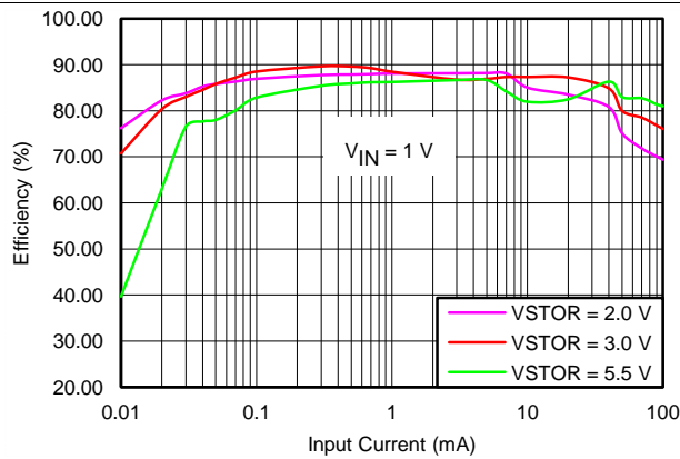
V_{IN} = 1 \text{ V} V_{IN\_DC} = sourcemeter configured with voltage source = 1.0 V and I_{COMP} varied from 0.01 mA to 100 mA V_{STOR} = sourcemeter configured to measure current and voltage source set to hold the V_{STOR} voltage = 2.0 V, 3.0 V or 5.5 V
