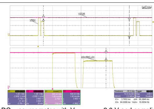
V_{IN\_DC} = sourcemeeter with V_{SOURCE} = 2.0\text{ V} and compliance of 43\text{ mA} V_{BAT} = sourcemeeter with V_{SOURCE} = 3.6\text{ V} and compliance of 1\text{ A}
