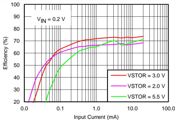
V_{IN} = 0.2 \text{ V} V_{IN\_DC} = sourcemeter configured with voltage source = 0.2 V and I_{COMP} varied from 0.01 mA to 100 mA V_{STOR} = sourcemeter configured to measure current and voltage source set to hold the V_{STOR} voltage = 2.0 V, 3.0 V or 5.5 V
