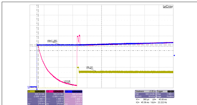
Sourcemeeter with V_{SOURCE} = 1.0\text{ V} and compliance of 8.5\text{ mA} subsequently applied to V_{IN\_DC} V_{BAT} = 0.1\text{ F} capacitor charged to 2.0\text{ V} Resistance on V_{STOR} = 100\text{ k}\Omega
