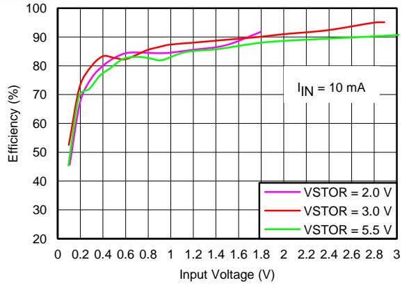
I_{IN} = 10 \text{ mA} V_{IN\_DC} = sourcemeter configured with I_{COMP} = 10 \text{ mA} and voltage source varied from 0.1 V to 3.0 V V_{STOR} = sourcemeter configured to measure current and voltage source set to hold the V_{STOR} voltage = 2.0 V, 3.0 V or 5.5 V
