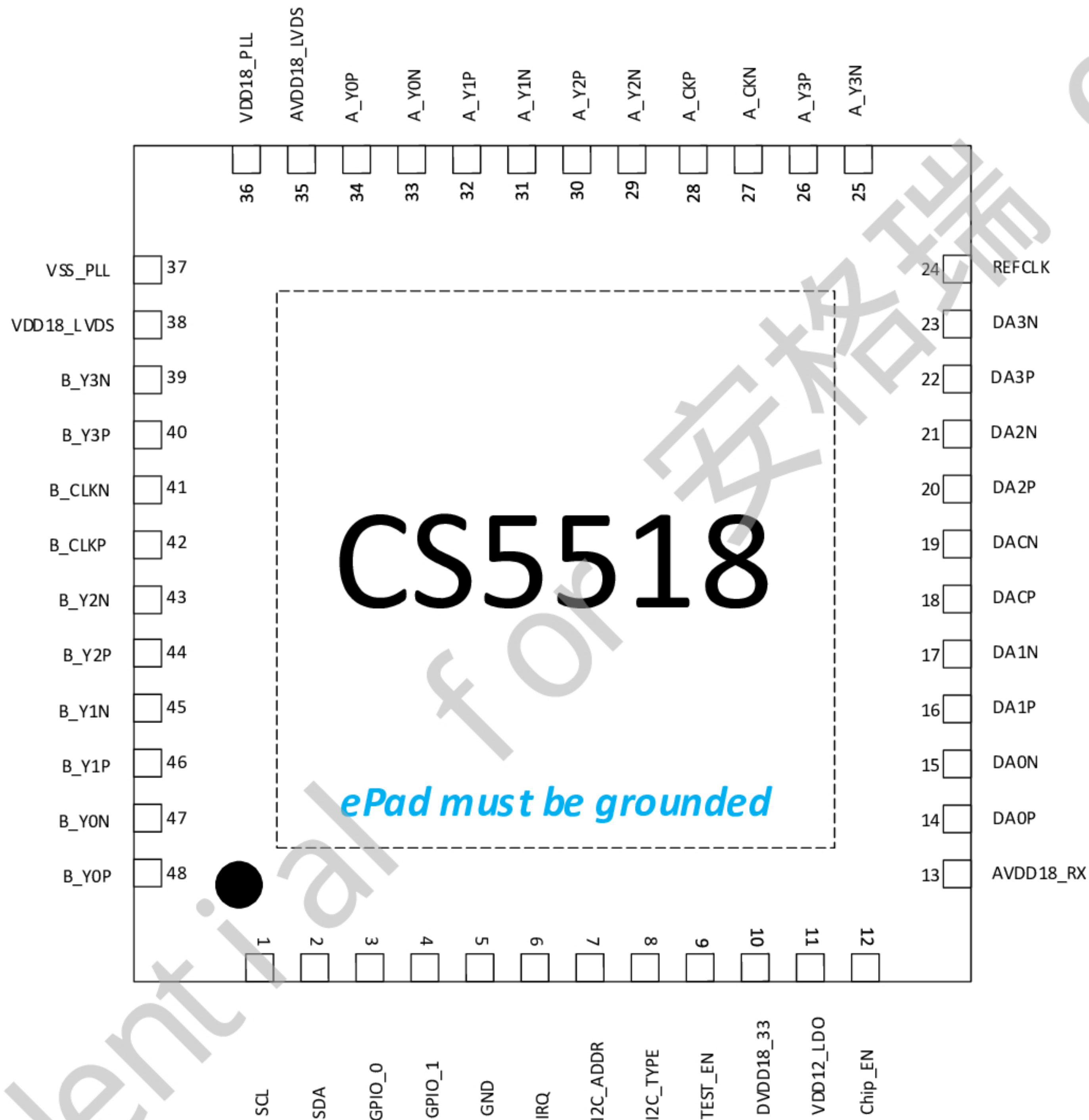
Figure 3-1 CS5518 Pin Layout
