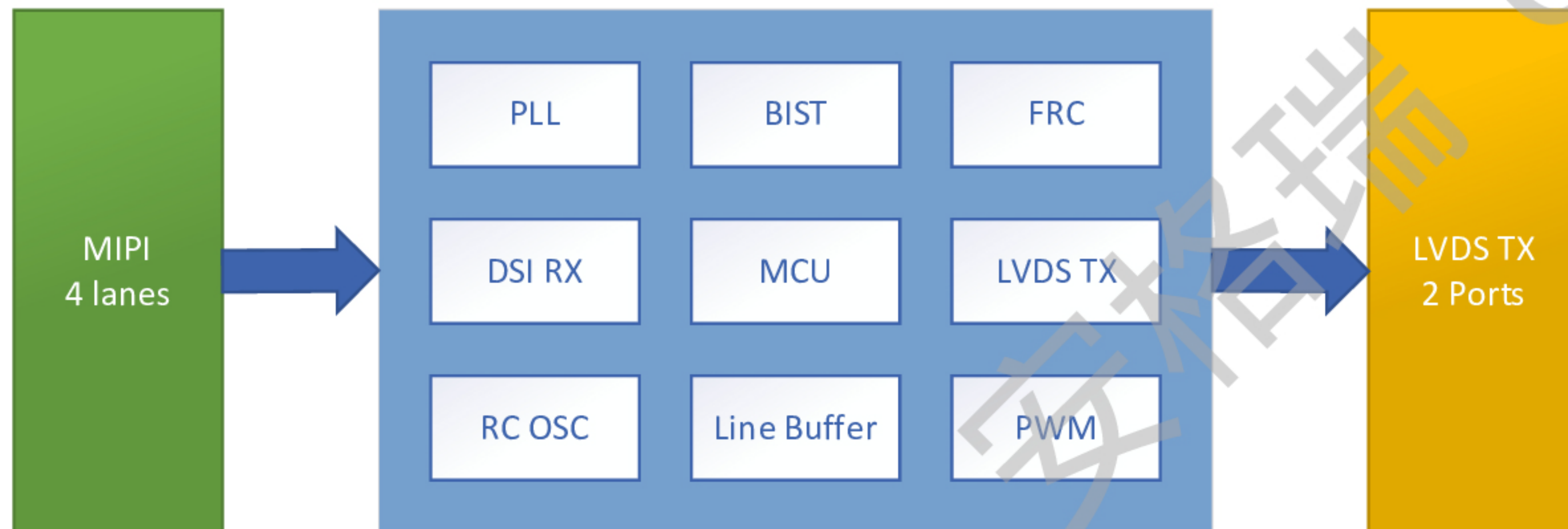
Figure 1-1 CS5518 Block Diagram
