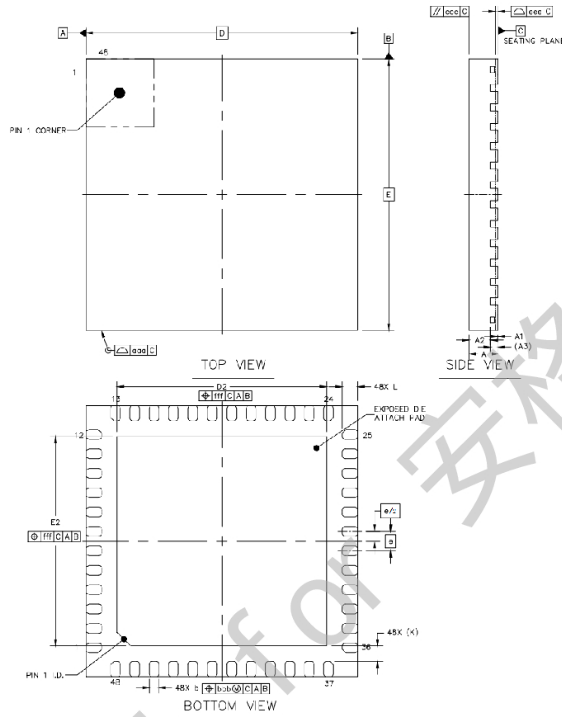
Figure 5-1 CS5518 Package Outline (QFN48 Leads 7x7mm)
