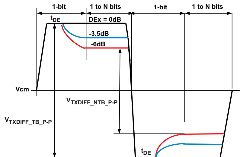
Figure 4. Output De-Emphasis Levels OSx = NC
