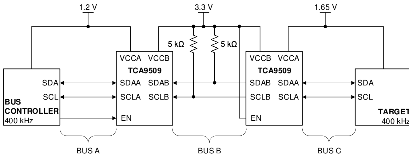
Figure 10-3. Typical Series Application, Two B-Sides Connected Together
