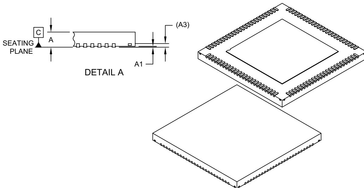
FIGURE 11-2: 100-VQFN PACKAGE (DIMENSIONS)
