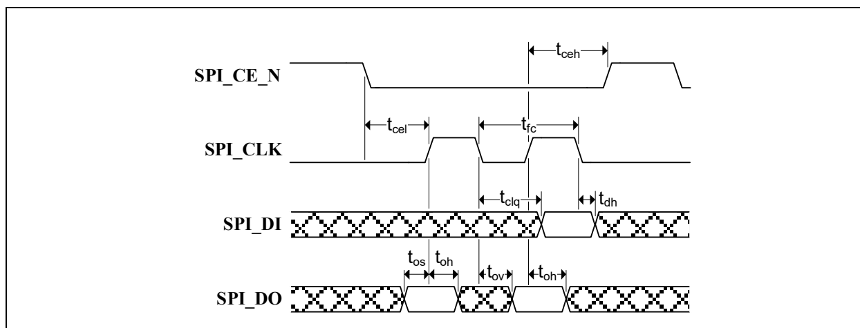
FIGURE 10-5: SPI TIMING
