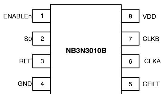
Figure 2. Pinout SOIC-8 (Top View)
