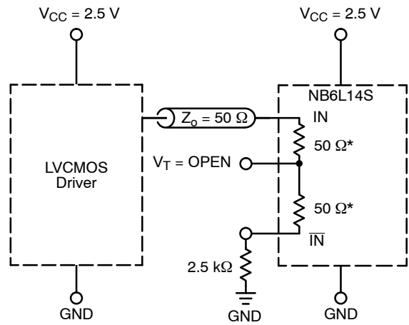
Figure 15. LVCMOS Interface
