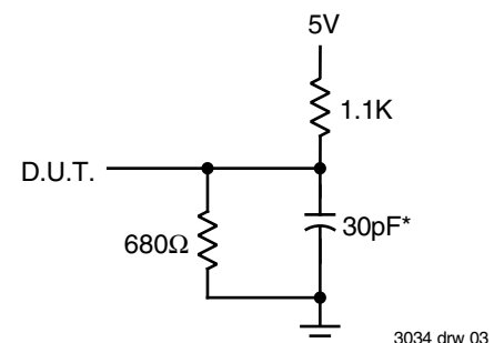
Figure 1. Output Load
