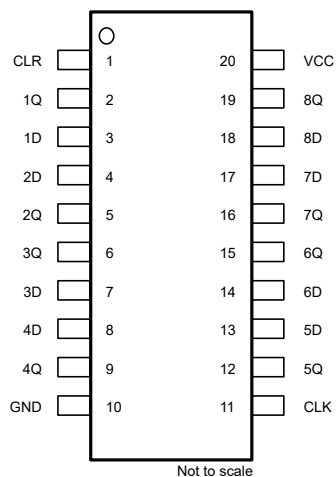
Figure 5-1. SN74LV273A DB, DGV, DW, NS, or PW Package, 20-Pin SSOP, TVSOP, SOP, or TSSOP (Top View)
