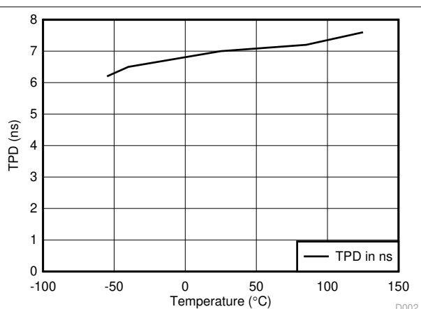
Figure 6-8. TPD vs Temperature
