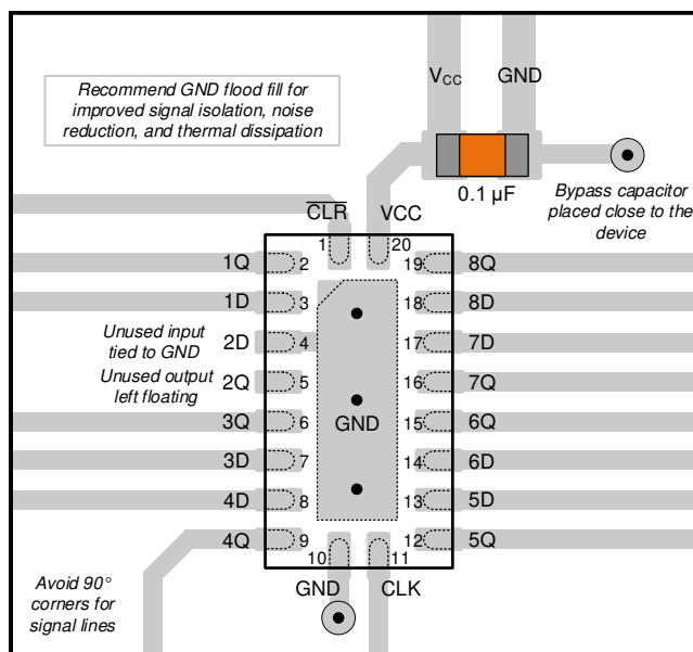
Figure 11-1. Layout Example for SN74LV273A in the RKS Package
