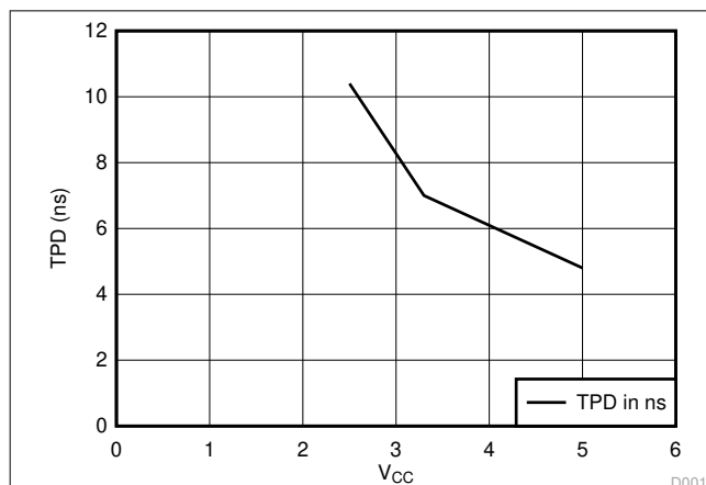
Figure 6-7. TPD vs V CC at 25°C
