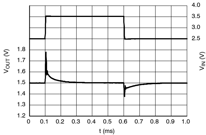
Figure 23. Line Transients, 1.5 V Version, t_R = t_F = 5 \mu\text{s} , I_{\text{OUT}} = 30 \text{ mA}
