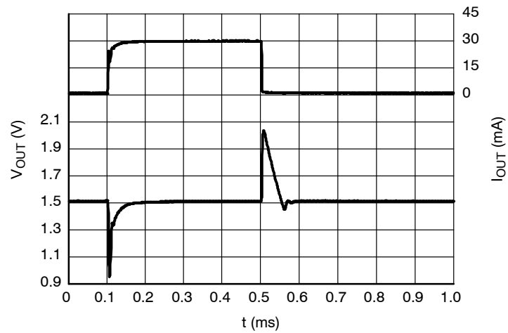
Figure 32. Load Transients, 1.5 V Version, I_{OUT} = 1 - 30 \text{ mA} , t_R = t_F = 0.5 \mu\text{s} , V_{IN} = 2.5 \text{ V}
