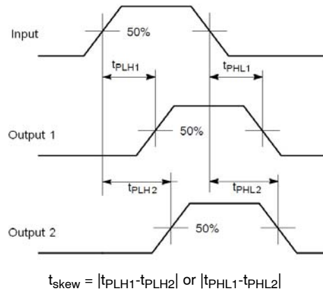
Figure 12. Bit-to-Bit and Channel-to-Channel Skew
