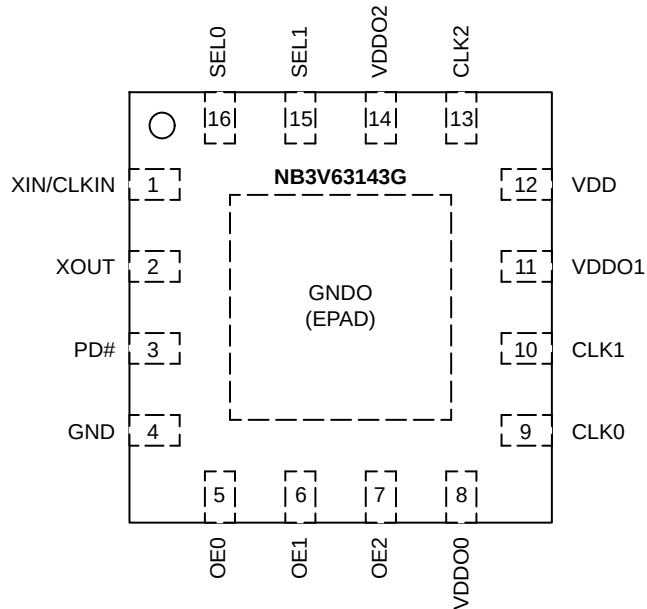
Figure 2. Pin Connections (Top View) – QFN16 (with EPAD)
