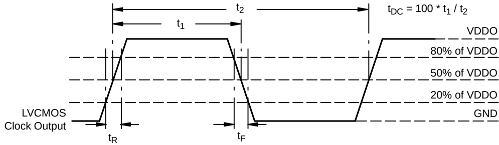
Figure 10. LVTMOS Measurement for AC Parameters
