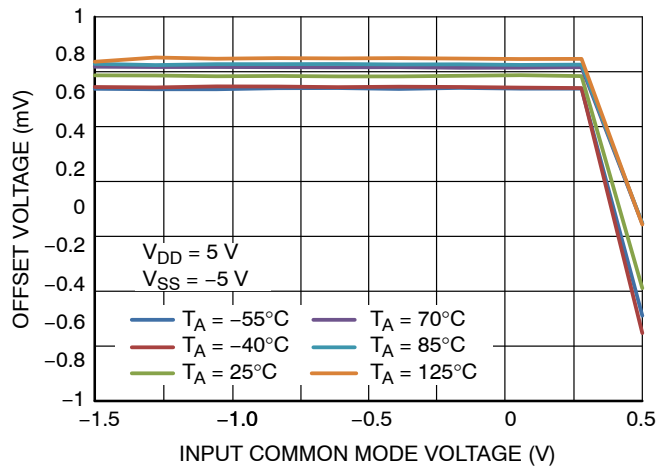
Figure 12. V_{OS} vs. V_{CM} ( V_S = 10 V)
