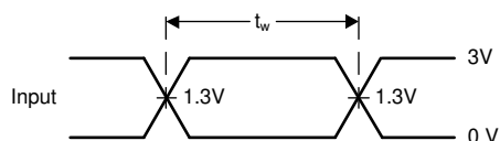
Figure 6-3. Voltage Waveforms, TTL-Compatible CMOS Inputs Pulse Duration
