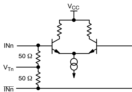
Figure 4. Input Structure
