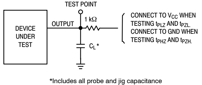
Figure 7. Test Circuit
