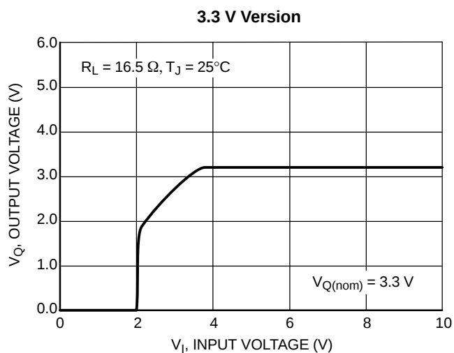
Figure 9. Output Voltage V_Q vs. Input Voltage V_I
