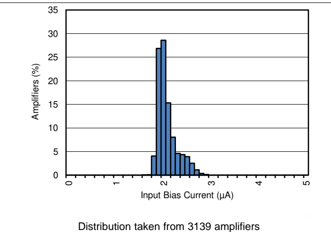
Figure 38. Input Bias Current Distribution
