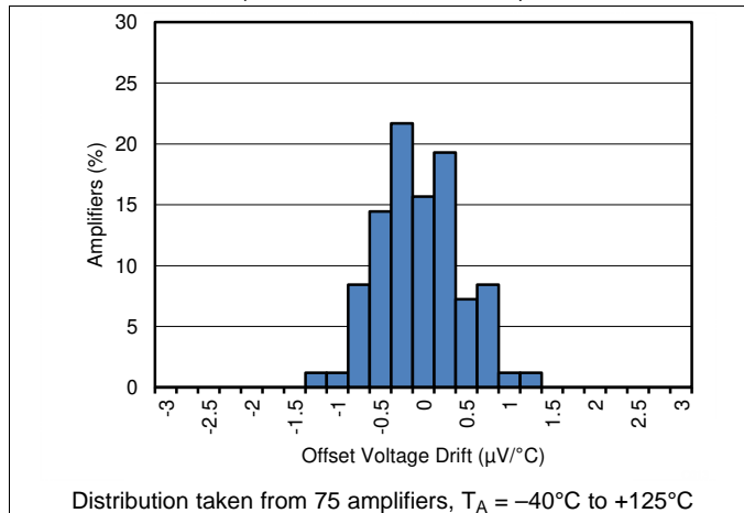
Figure 37. Input Offset Voltage Drift Distribution
