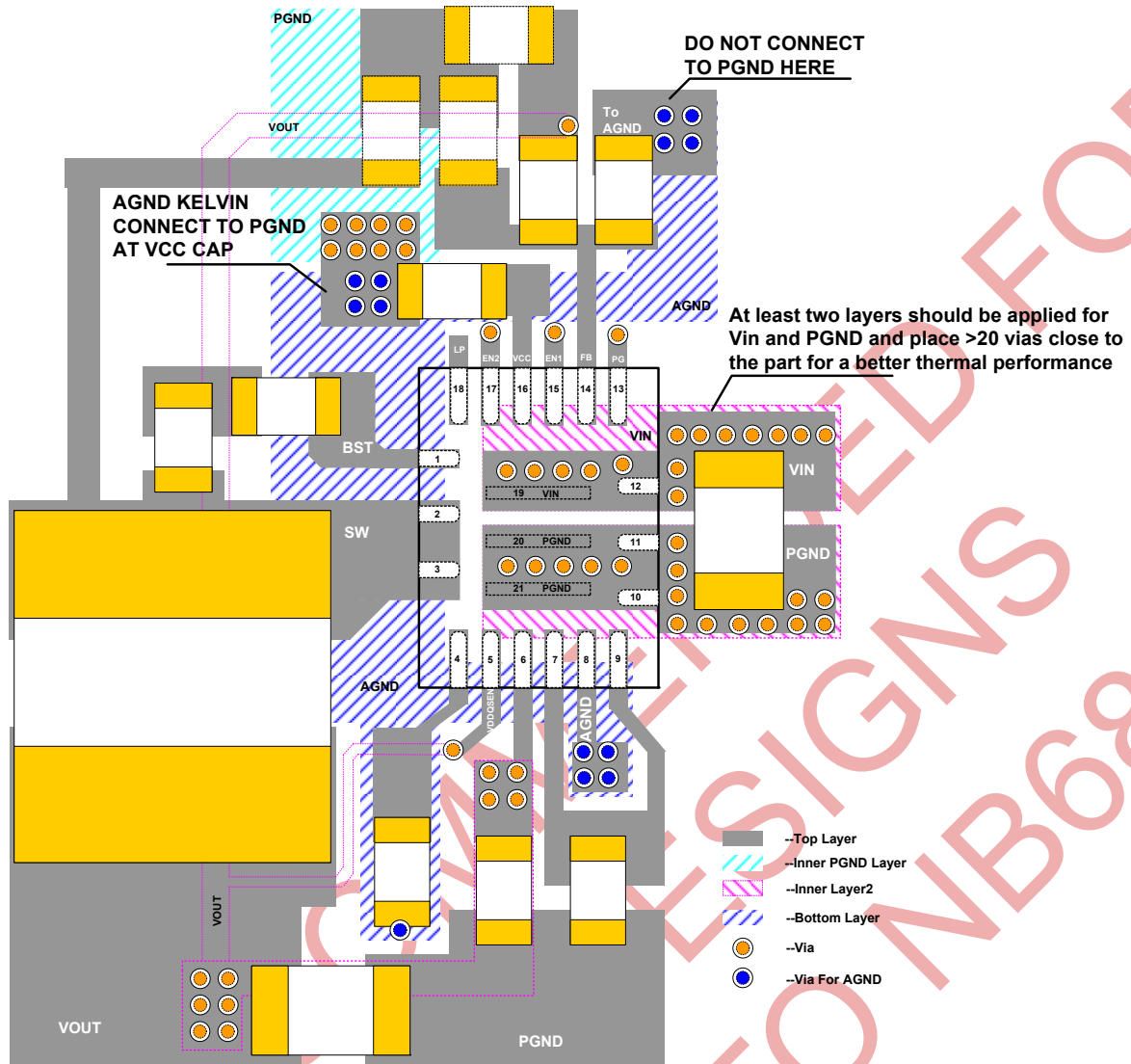
Figure 13—Recommend Layout
