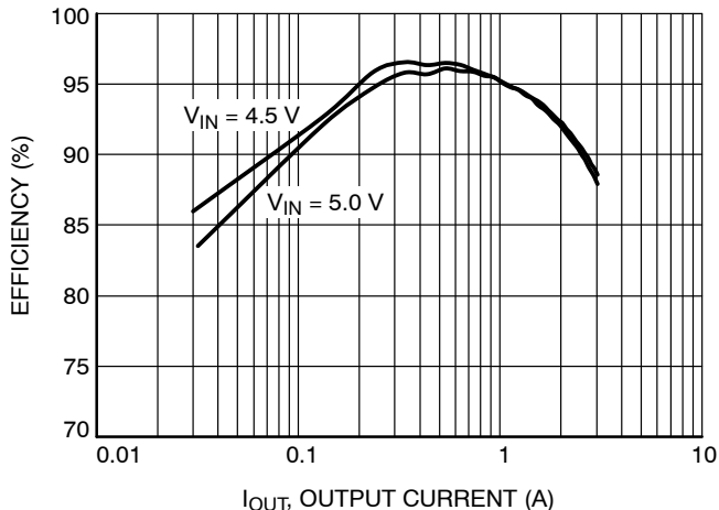
Figure 3. Efficiency vs. Output Current (3.3 V)
