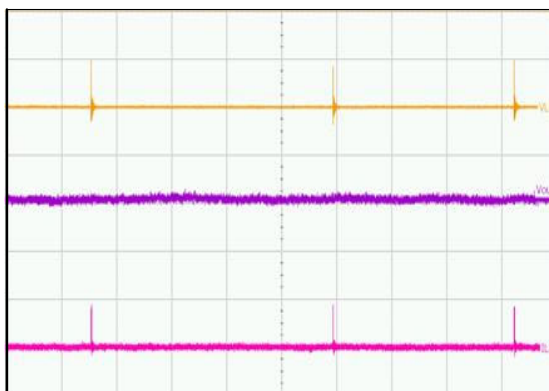
(VIN = 5 V, VOUT = 1.05 V, IOULT = 0 A) Upper Trace: LX Pin Switching Waveforms, 5 V / div Middle Trace: Output Voltage, 20 mV / div Lower Trace: Inductor Current, 100 mA / div Time = 20 \mu s / div
