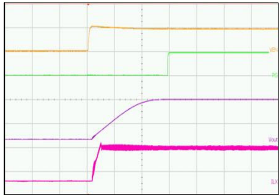
(VIN = 5 V, VOUT = 1.8 V, IOU T = 3 A, CSS = 4.7 nF) Upper Trace: Enable Pin Voltage, 5 V / div Second Trace: Power Good Pin Voltage, 5 V / div Third Trace: Output Voltage, 2 V / div Lower Trace: Inductor Current, 2 A / div Time = 2 ms / div
