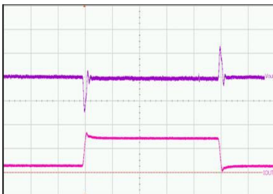
(VIN = 5 V, VOUT = 1.05 V, IOULT = 0.5 A to 3.0 A) Upper Trace: Output Voltage, 50 mV / div Lower Trace: Output Current, 2 A / div Time = 200 \mu s/div
