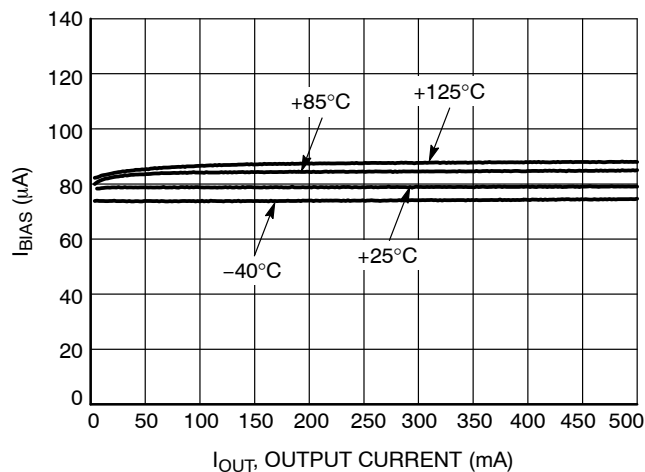
Figure 9. BIAS Pin Current vs. I_{OUT} and Temperature T_J
