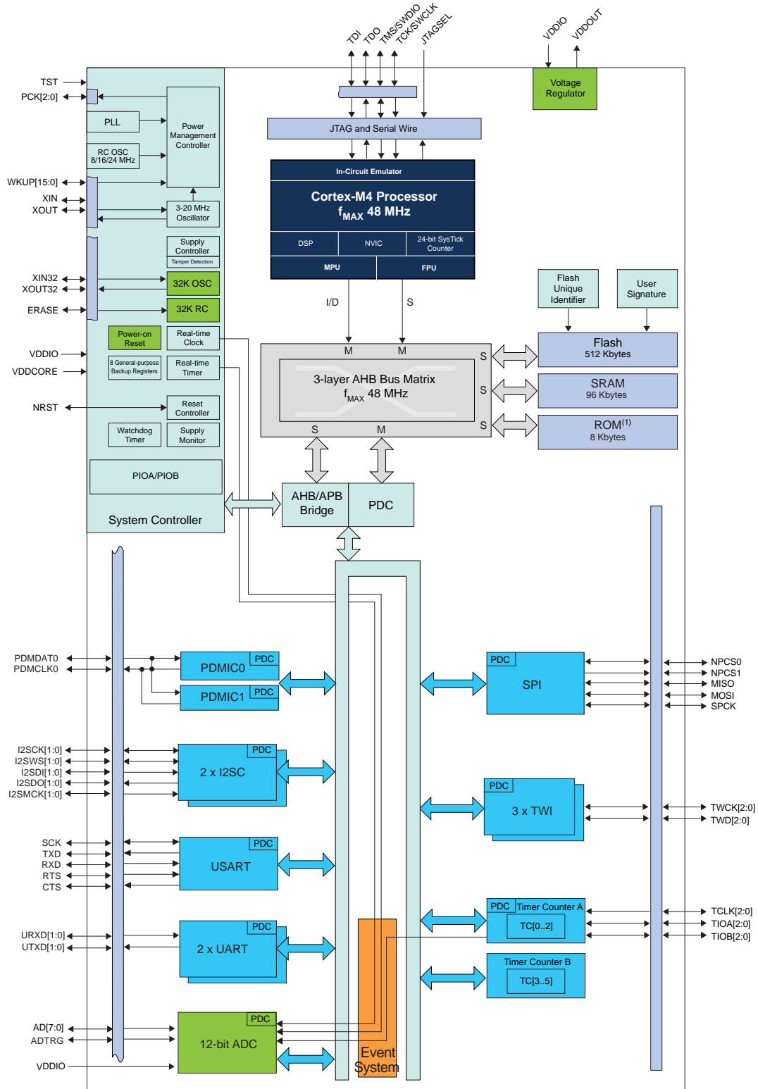
Figure 2-1. SAM G53 Block Diagram
