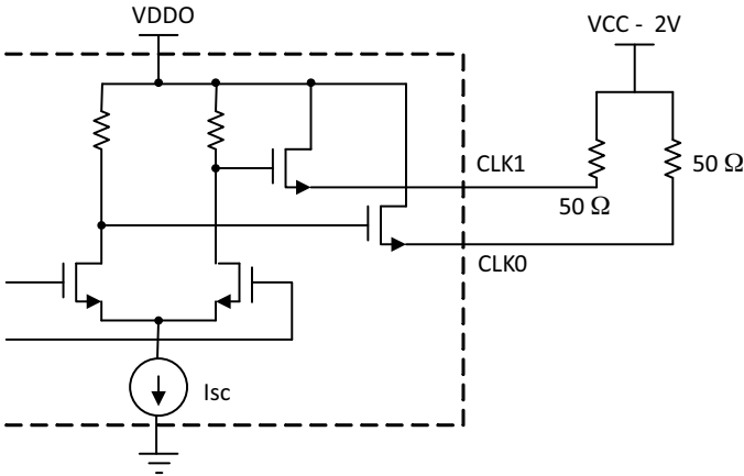
Figure 19. Simplified LVPECL Output Structure with Termination
