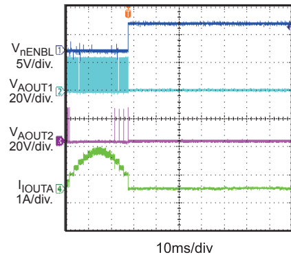
Disable-Eighth Step
