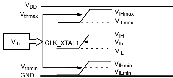
Figure 5. V_{th} Diagram
