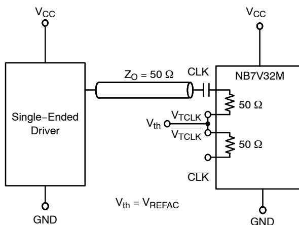
Figure 16. Capacitor-Coupled Single-Ended Interface ( V_{TCLK}/\overline{V_{TCLK}} Connected to V_{REFAC} ; V_{REFAC} Bypassed to Ground with 0.1 \mu F Capacitor)
