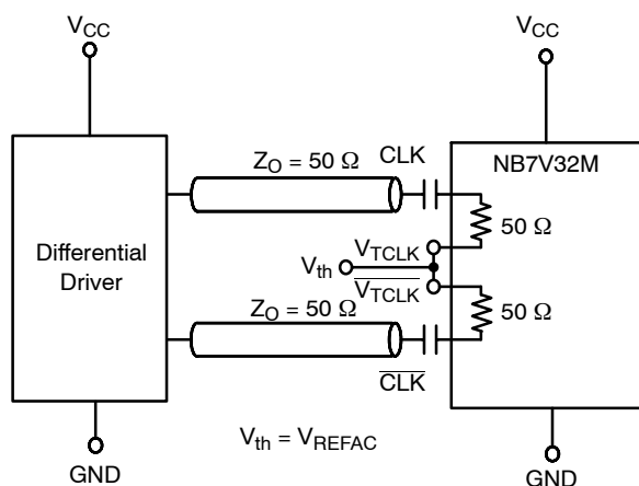
Figure 15. Capacitor-Coupled Differential Interface ( V_{TCLK}/\overline{V_{TCLK}} Connected to V_{REFAC} ; V_{REFAC} Bypassed to Ground with 0.1 \mu F Capacitor)
