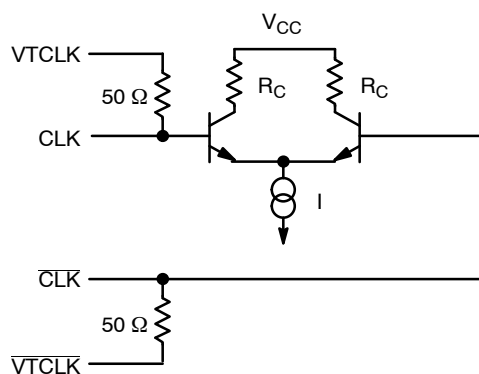
Figure 4. Input Structure
