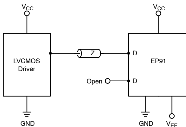
Figure 11. Standard LVC MOS Interface ( \overline{D} will default to V_{CC}/2 when left open. A reference voltage of V_{CC}/2 should be applied to D input, if \overline{D} is interfaced to CMOS signals)
