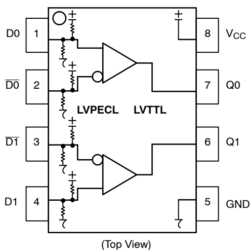
Figure 1. Logic Diagram and 8-Lead Pinout
