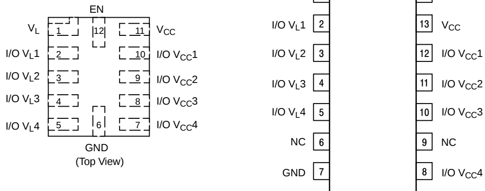
Figure 1. Pin Assignments
