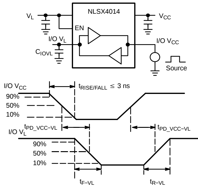
Figure 6. Driving I/O V_{CC} Test Circuit and Timing
