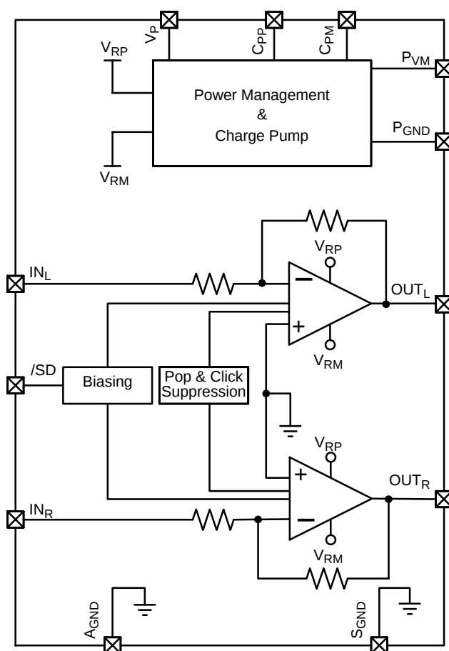
Figure 1. Block Diagram
