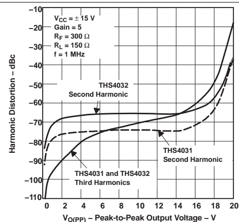
Figure 18. Harmonic Distortion vs Peak-to-Peak Output Voltage
