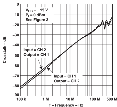
Figure 14. THS4032 Crosstalk vs Frequency
