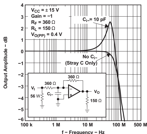
Figure 52. Output Amplitude vs Frequency
