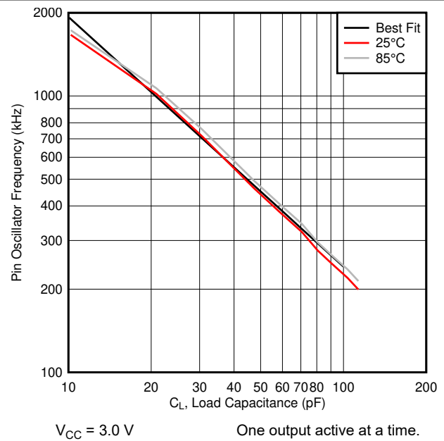
Figure 8-13. Typical Oscillation Frequency vs Load Capacitance
