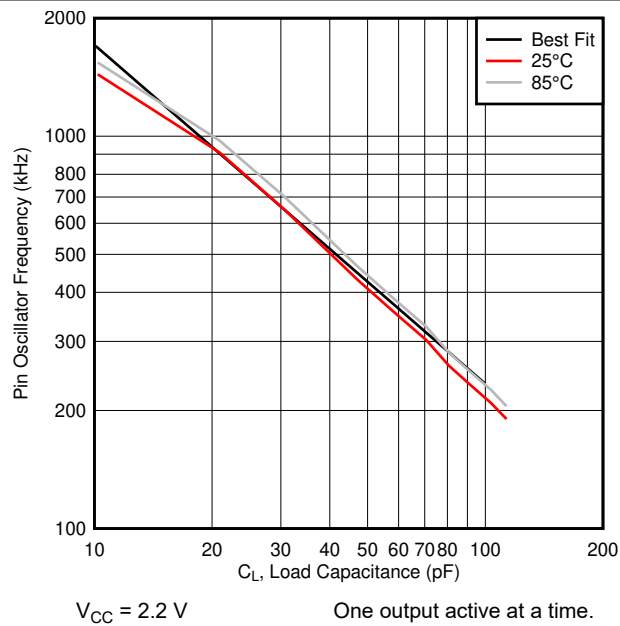
Figure 8-12. Typical Oscillation Frequency vs Load Capacitance
