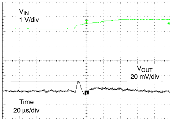
Figure 17. 3.0 V to 3.6 V Line Transient (Risettime = 50\text{ }\mu\text{s} , V_{OUT} = 1.2\text{ V} , I_{OUT} = 100\text{ mA} , T_A = 25^\circ\text{C} )
