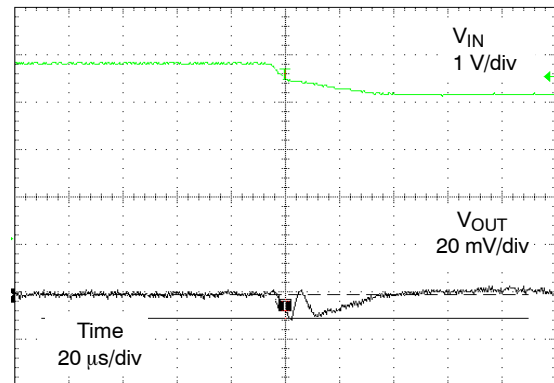
Figure 18. 3.6 V to 3.0 V Line Transient (Risettime = 50\text{ }\mu\text{s} , V_{OUT} = 1.2\text{ V} , I_{OUT} = 100\text{ mA} , T_A = 25^\circ\text{C} )
