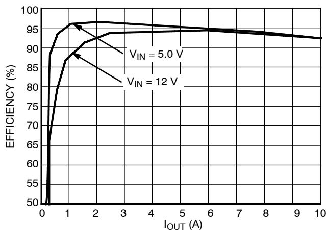
Figure 2. Efficiency
