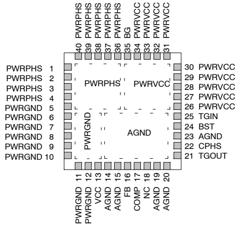
Figure 4. Pin Connections
