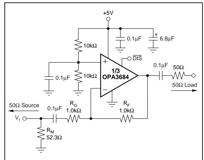
FIGURE 4. AC-Coupled, G = -1\text{V/V} , Single-Supply Specifications and Test Circuit.
