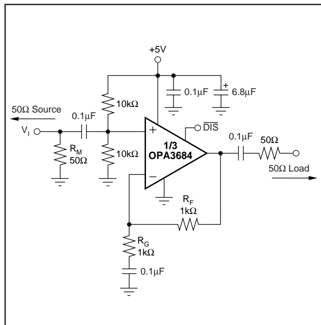
FIGURE 3. AC-Coupled, G = +2\text{V/V} , Single-Supply Specifications and Test Circuit.
