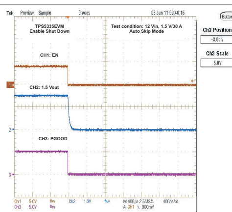
Figure 8-4. Enable Turn-off
