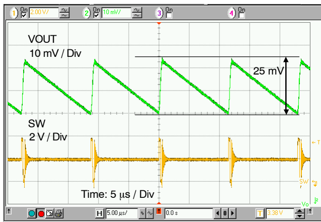
Figure 14. Output Ripple Voltage in PFM Mode ( V_{IN} = 3.6\text{ V} , V_{OUT} = 1.8\text{ V} , I_{OUT} = 10\text{ mA} , L = 1\text{ }\mu\text{H} , C_{OUT} = 10\text{ }\mu\text{F} )
