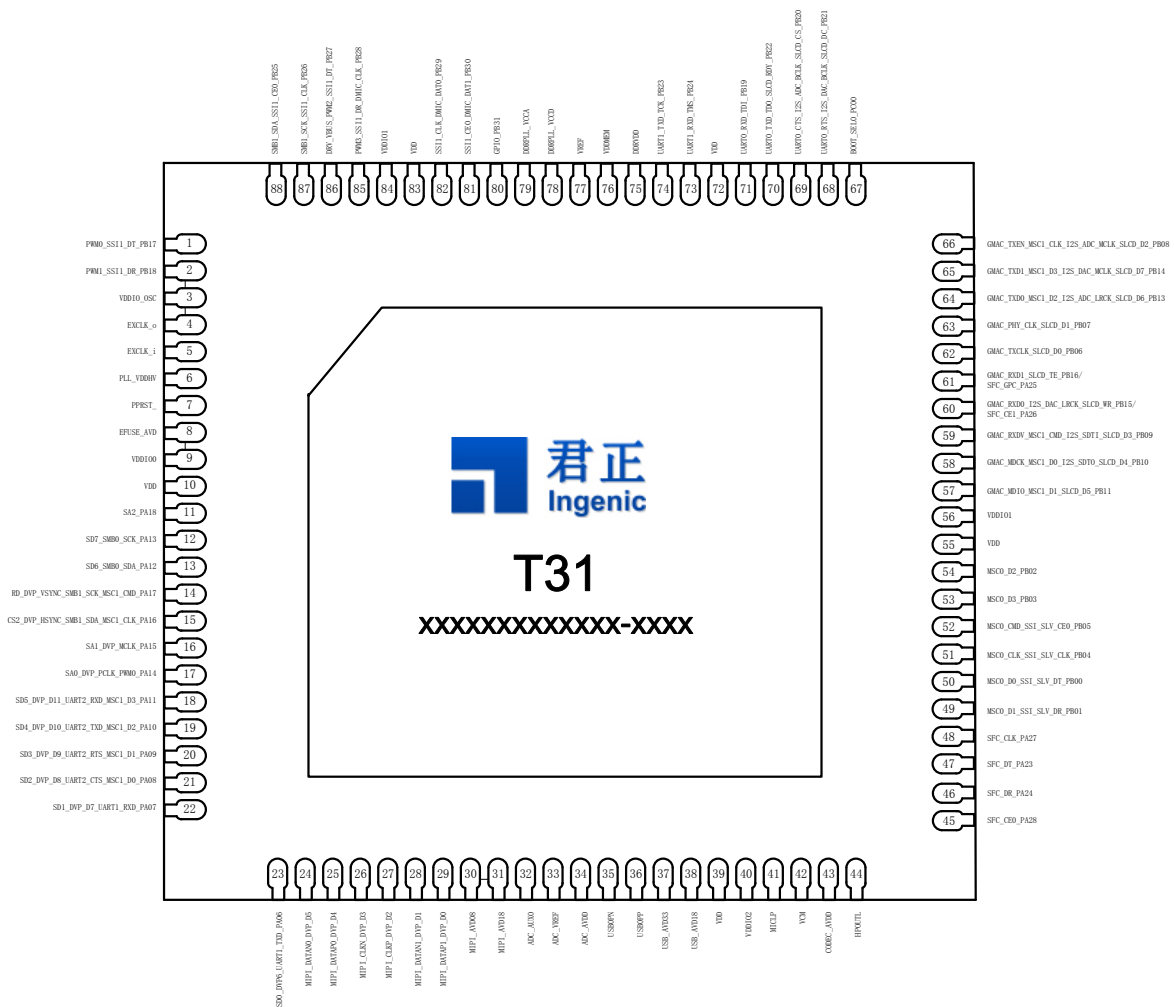
Figure 2-2 T31ZL pin to ball assignment
