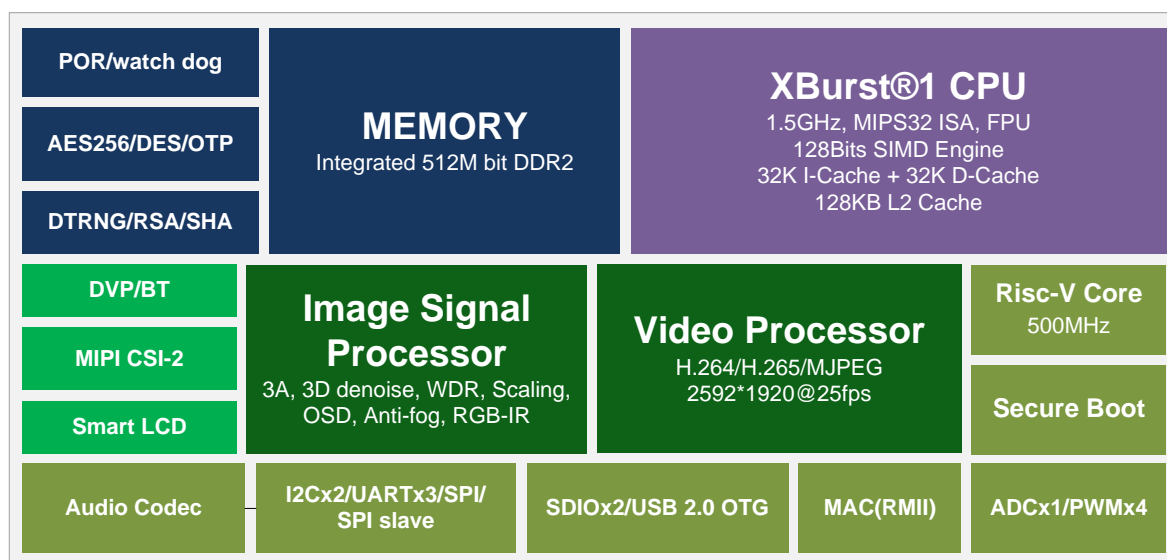
Figure 1-1 T31ZL Diagram
