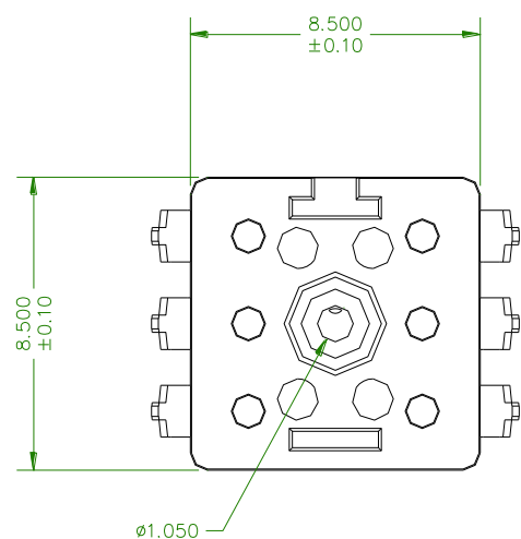
BM66 (Unit : mm )
