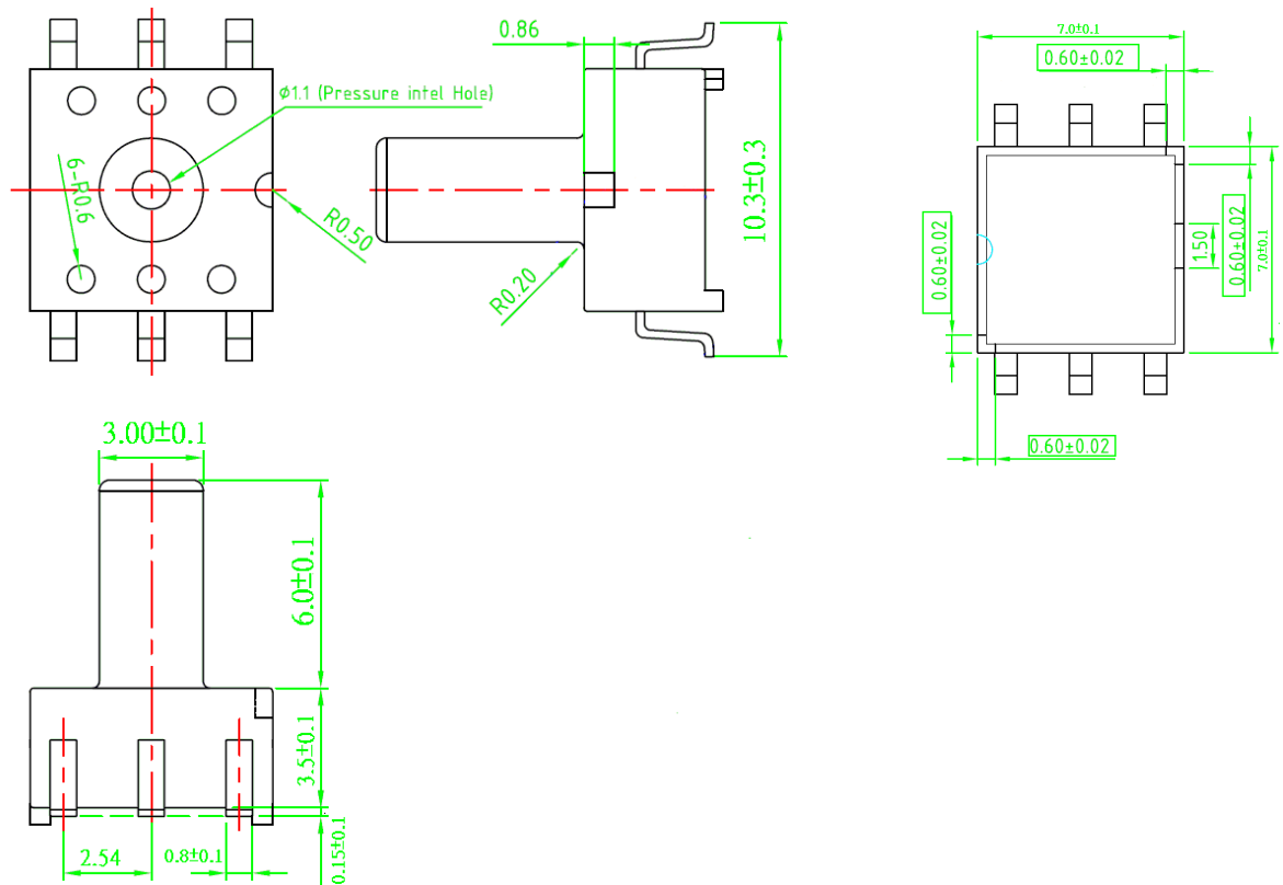
BM77 (Unit : mm )
