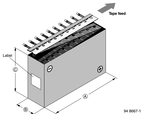
Fig. 12 - Tape Direction
