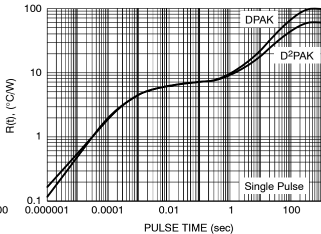
Figure 38. NCV8675 @ PCB Cu Area 100 \text{mm}^2 PCB Cu thk 1 oz
