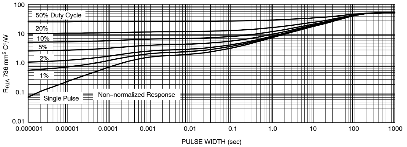
Figure 22. Duty Cycle for 1" Spreaders Boards, DPAK 5-Lead
