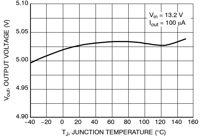
Figure 7. Output Voltage vs. Temperature
