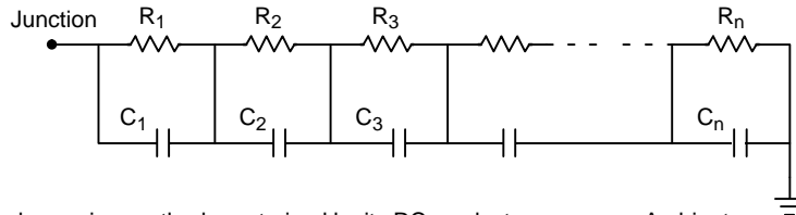
Figure 30. Non-Grounded Capacitor Thermal Ladder ("Foster" Ladder)
